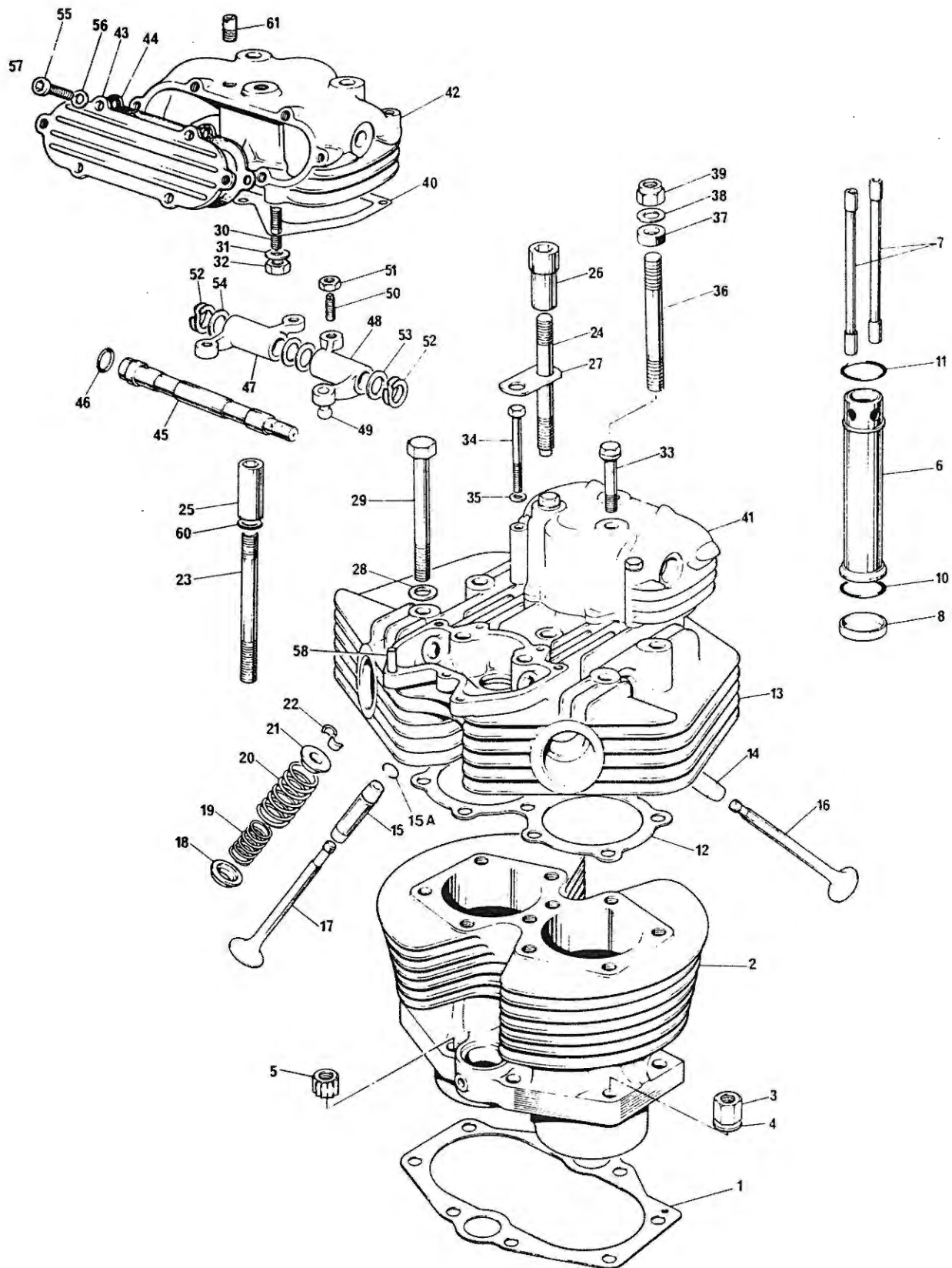
Fig. 5. CYLINDER BLOCK AND HEAD
