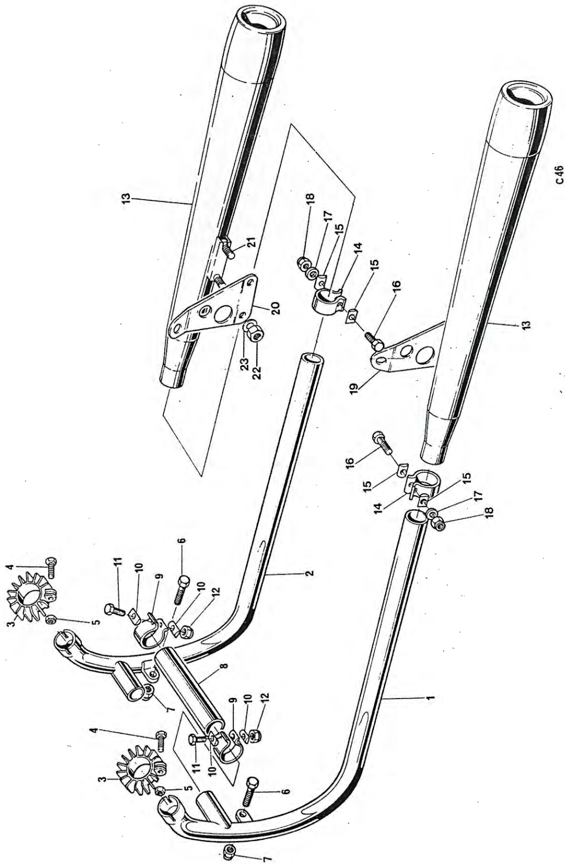
Fig. 12. EXHAUST SYSTEM
