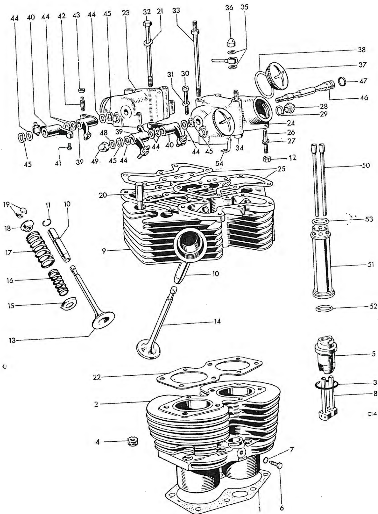
Fig. 6. CYLINDER BLOCK AND HEAD
