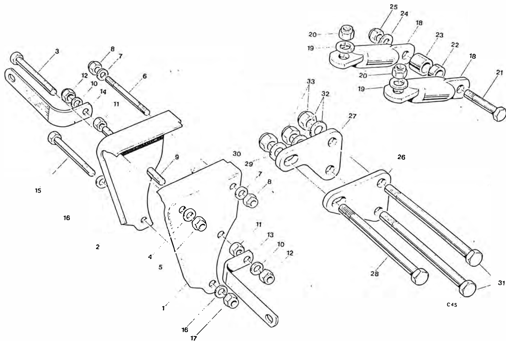
Fig. 16. MOTOR FITTINGS
