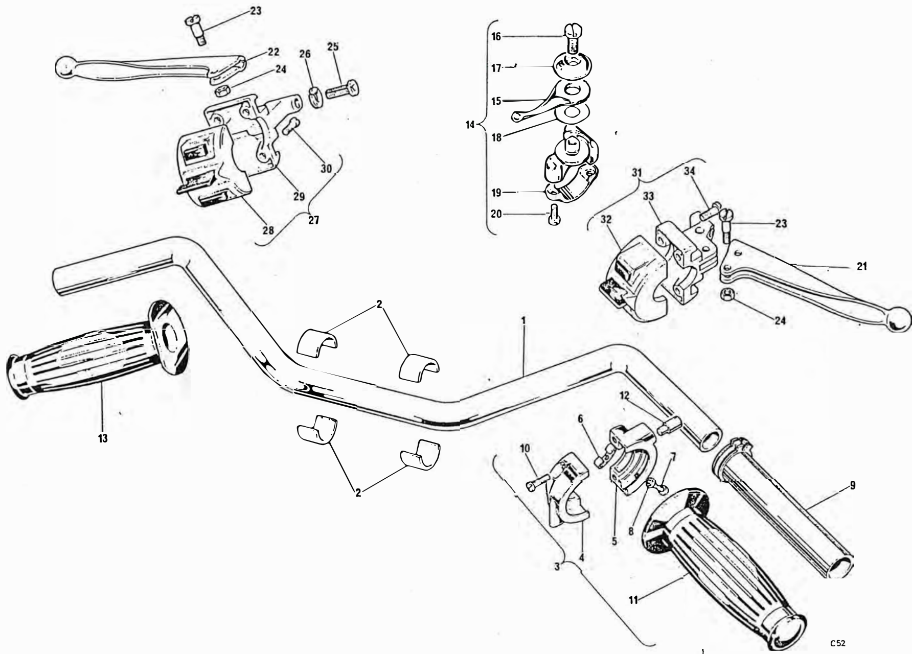
Fig. 30. HANDLEBAR AND CONTROL LEVERS
