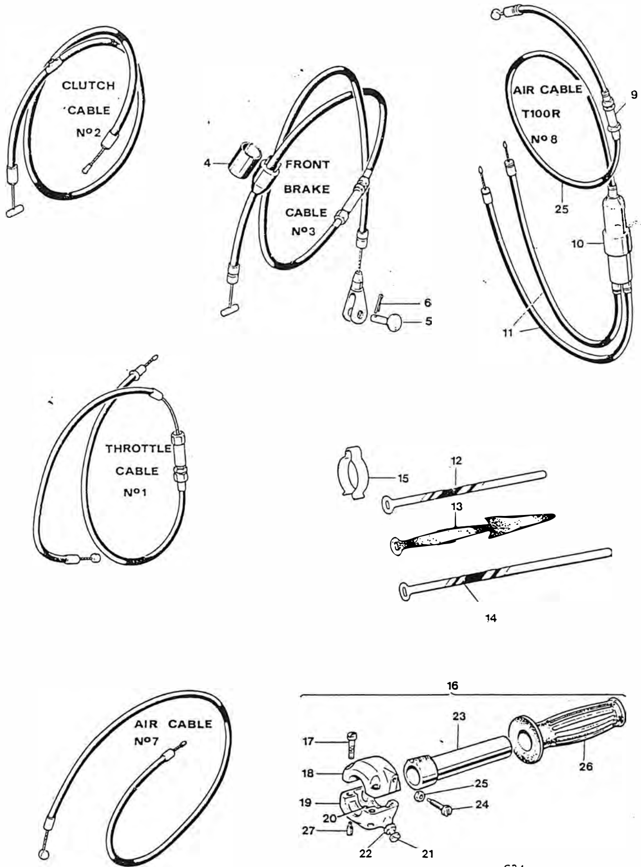
Fig. 32. CONTROL CABLES
