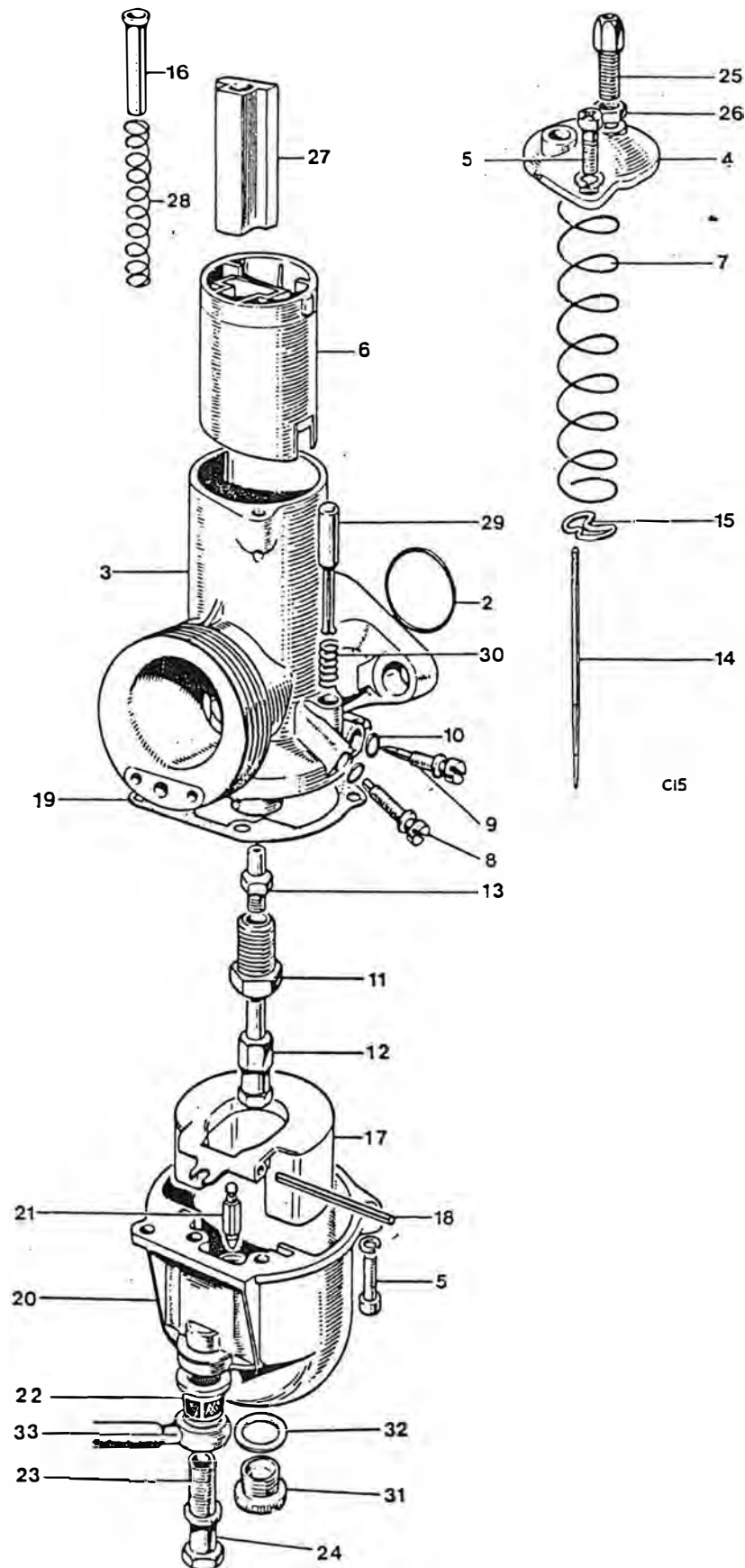
Fig. 5. CARBURETOR T100C
