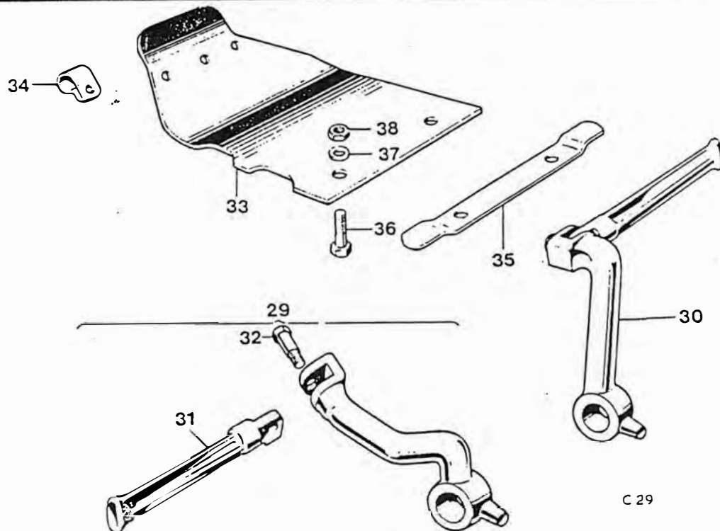
Fig. 17. EXHAUST PIPES, UNDERSHIELD AND FOOTPEGS (T100C)
