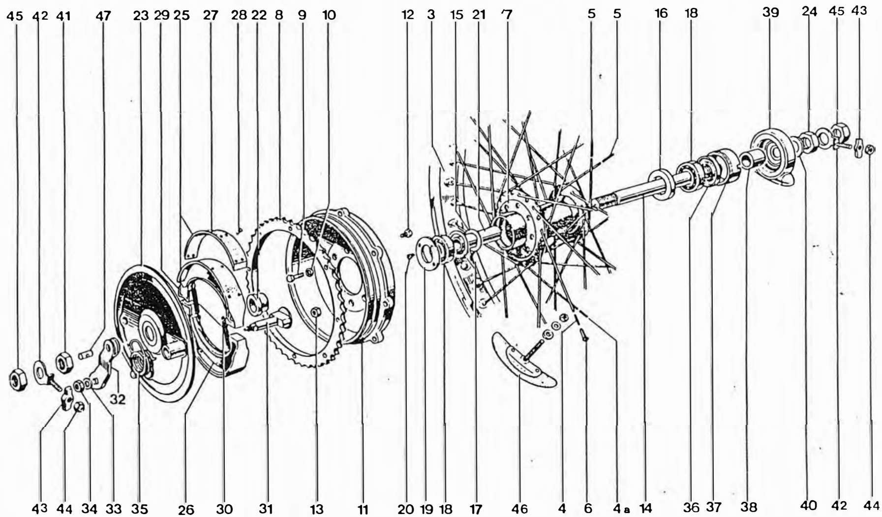
Fig. 32. REAR WHEEL
