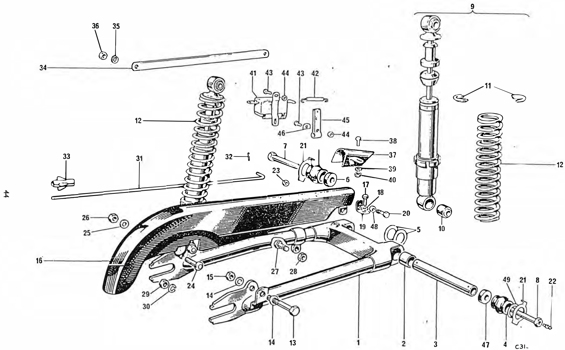
Fig. 19. SWINGING ARM, SUSPENSION UNITS AND CHAINGUARD
