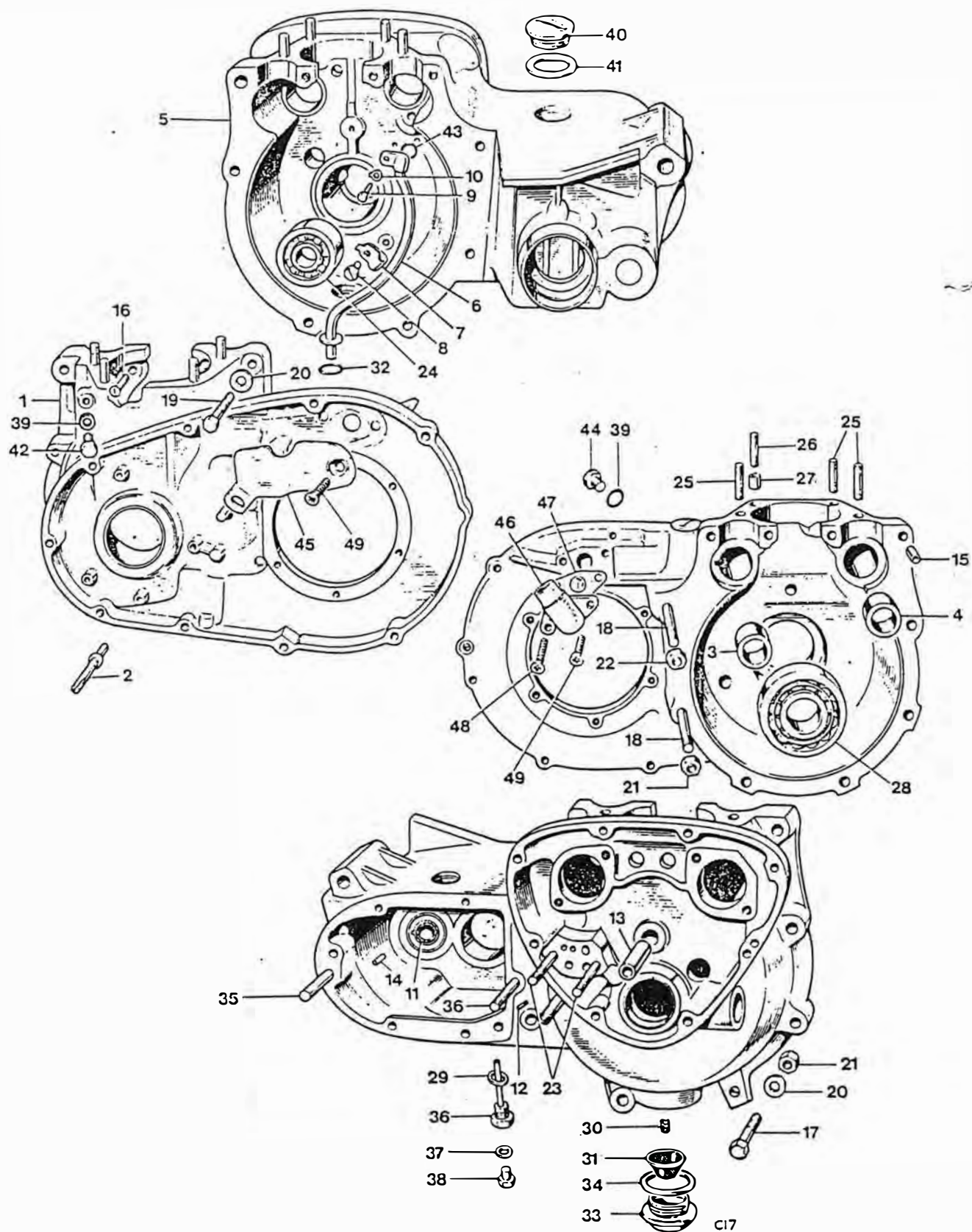
Fig. 2 CRANKCASE
