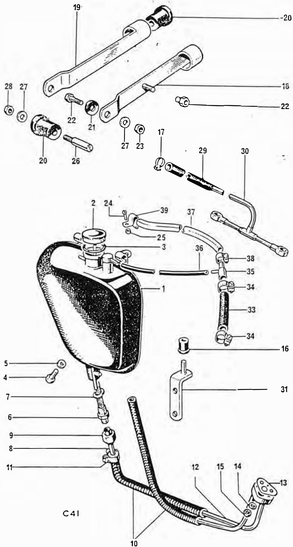
Fig. 28. OIL TANK
