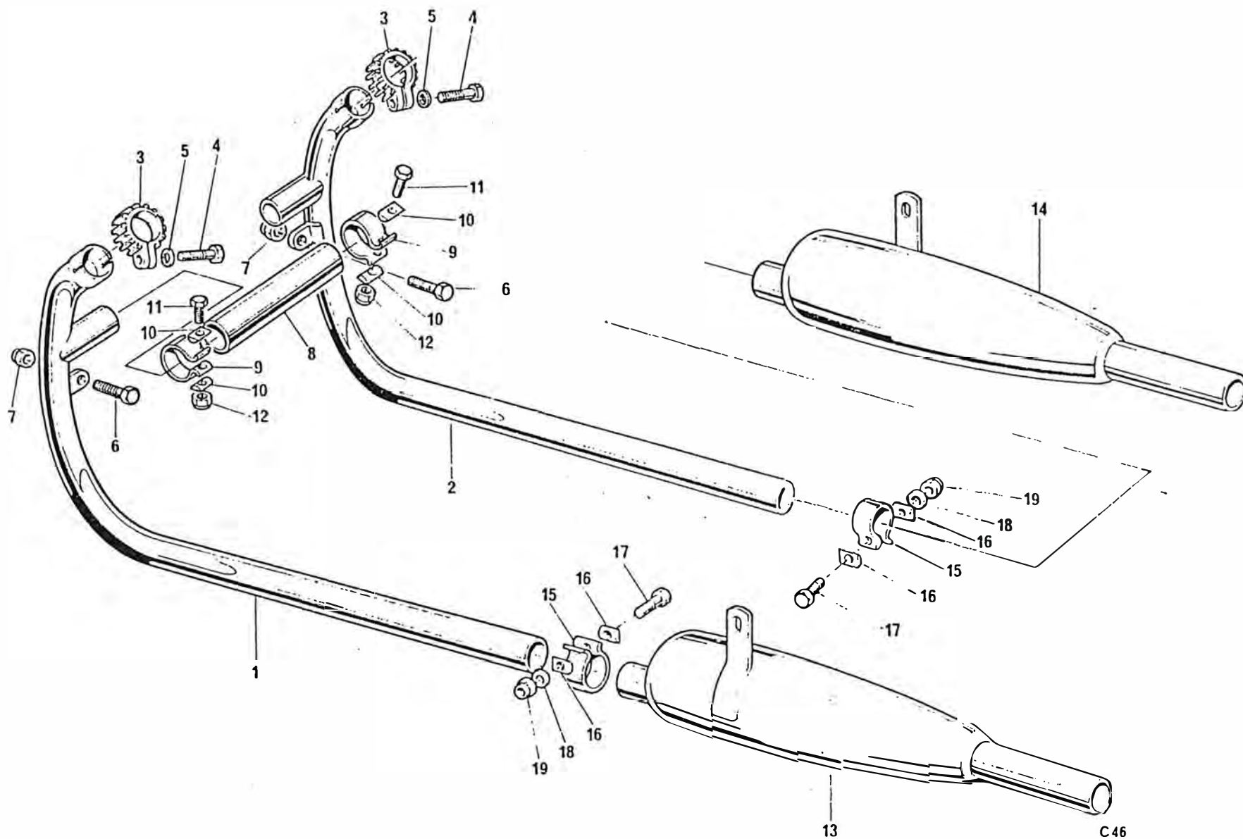
Fig. 15. EXHAUST SYSTEM
