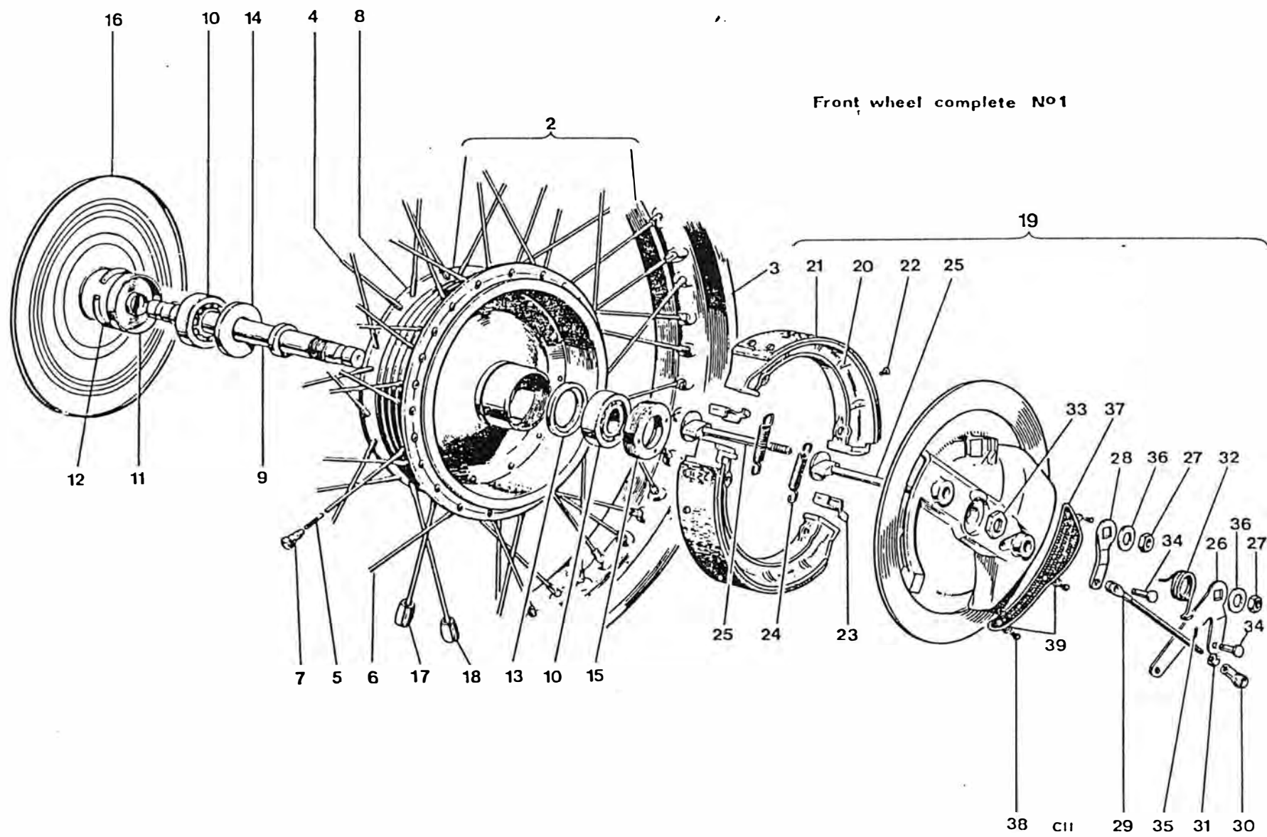
Fig. 21. FRONT WHEEL T100R
